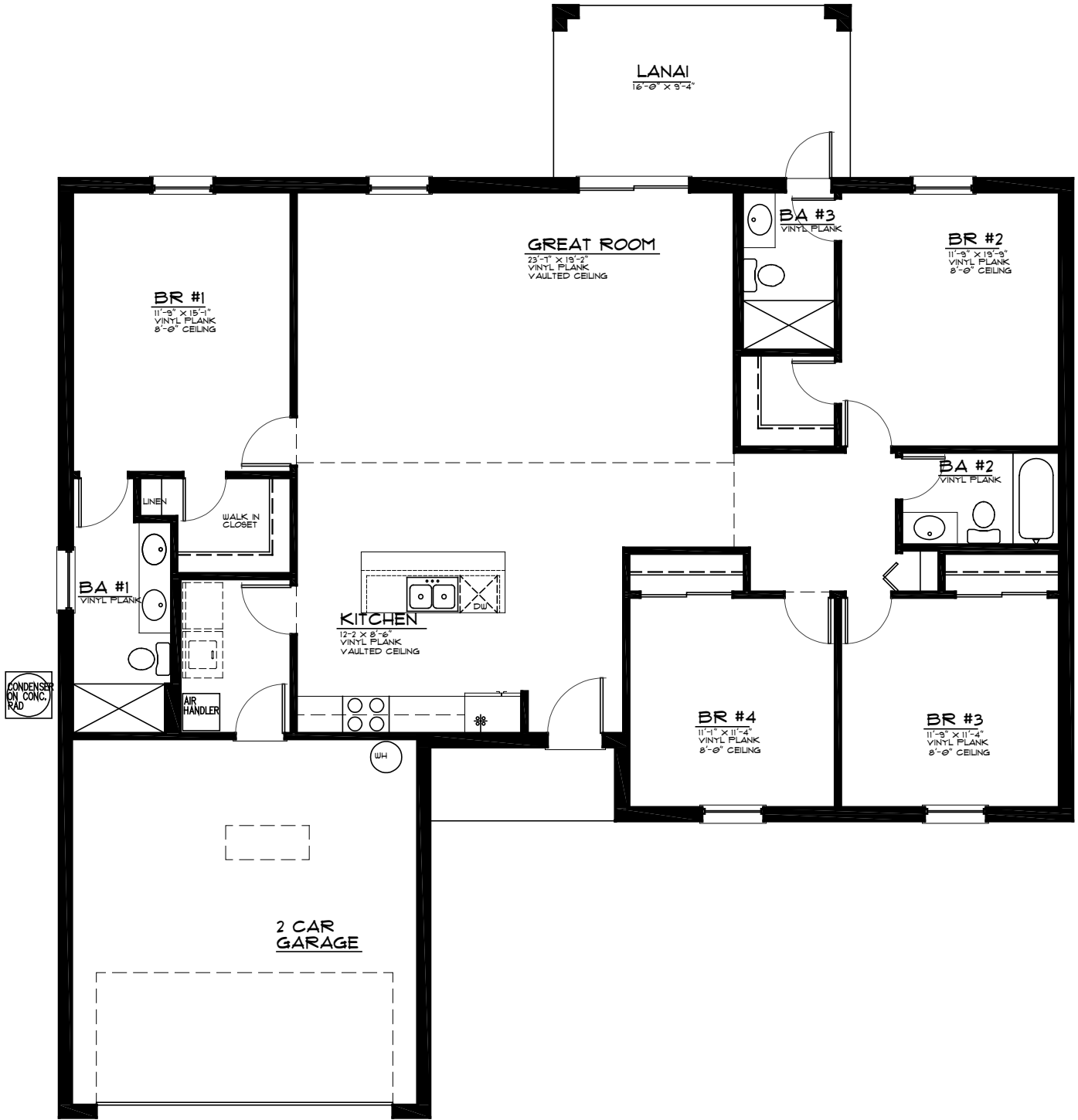
FIRST FLOOR PLAN 1761 HEATED SQUARE FEET
